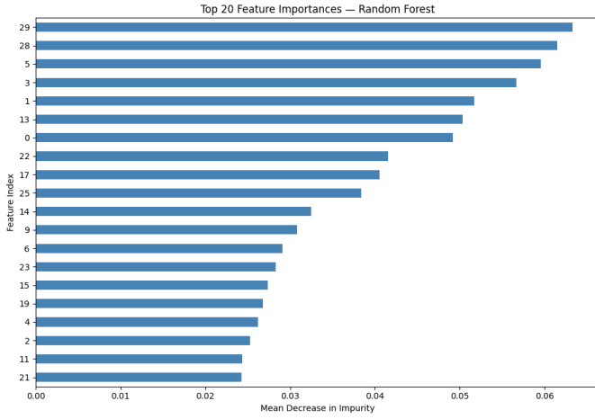
Fig. 1. Random Forest Feature Importance
